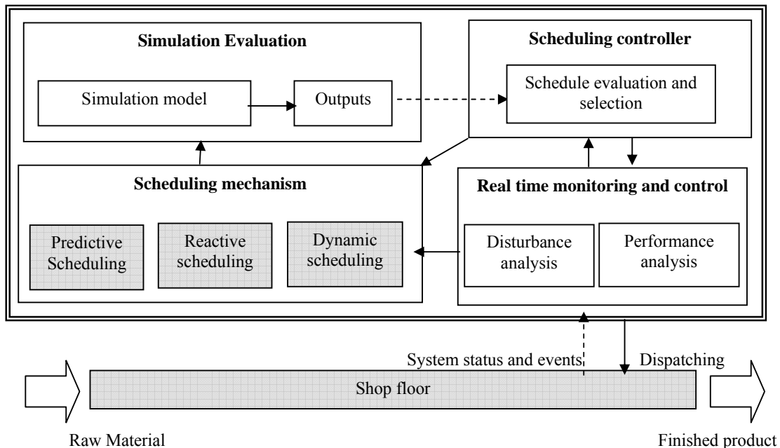
Figure 1: Reactive Scheduling Mechanism for dynamic discrete manufacturing
